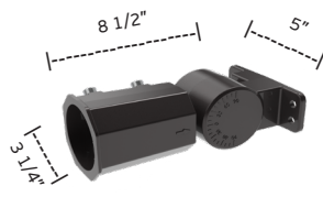
SF- Slip-Fitter Mount
